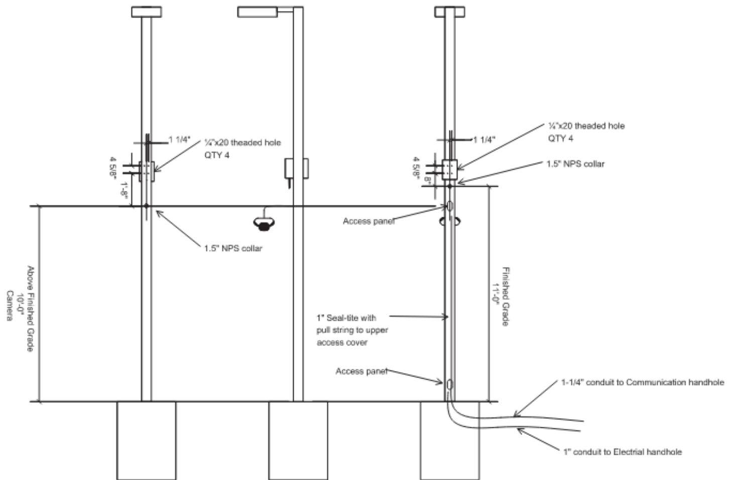
Typical Security Camera/WiFi Parking Light Pole
